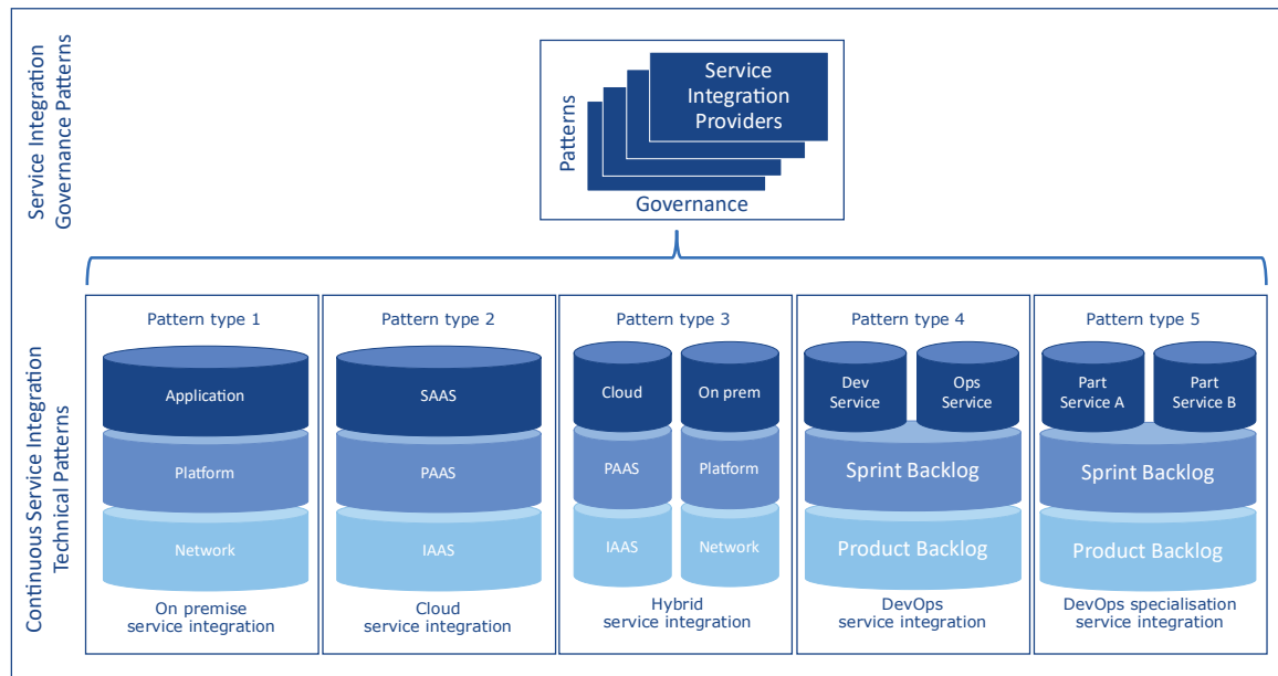
Figure 1-2, Continuous Service Integration patterns.
